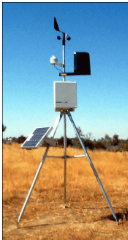
110-WS-25N Modular Weather Station with Optional Solar Panel Charger
