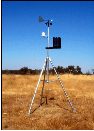
110-WS-25 Modular Weather Station
