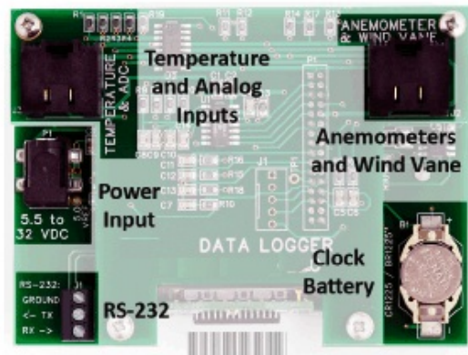
Data Logger circuit board.
